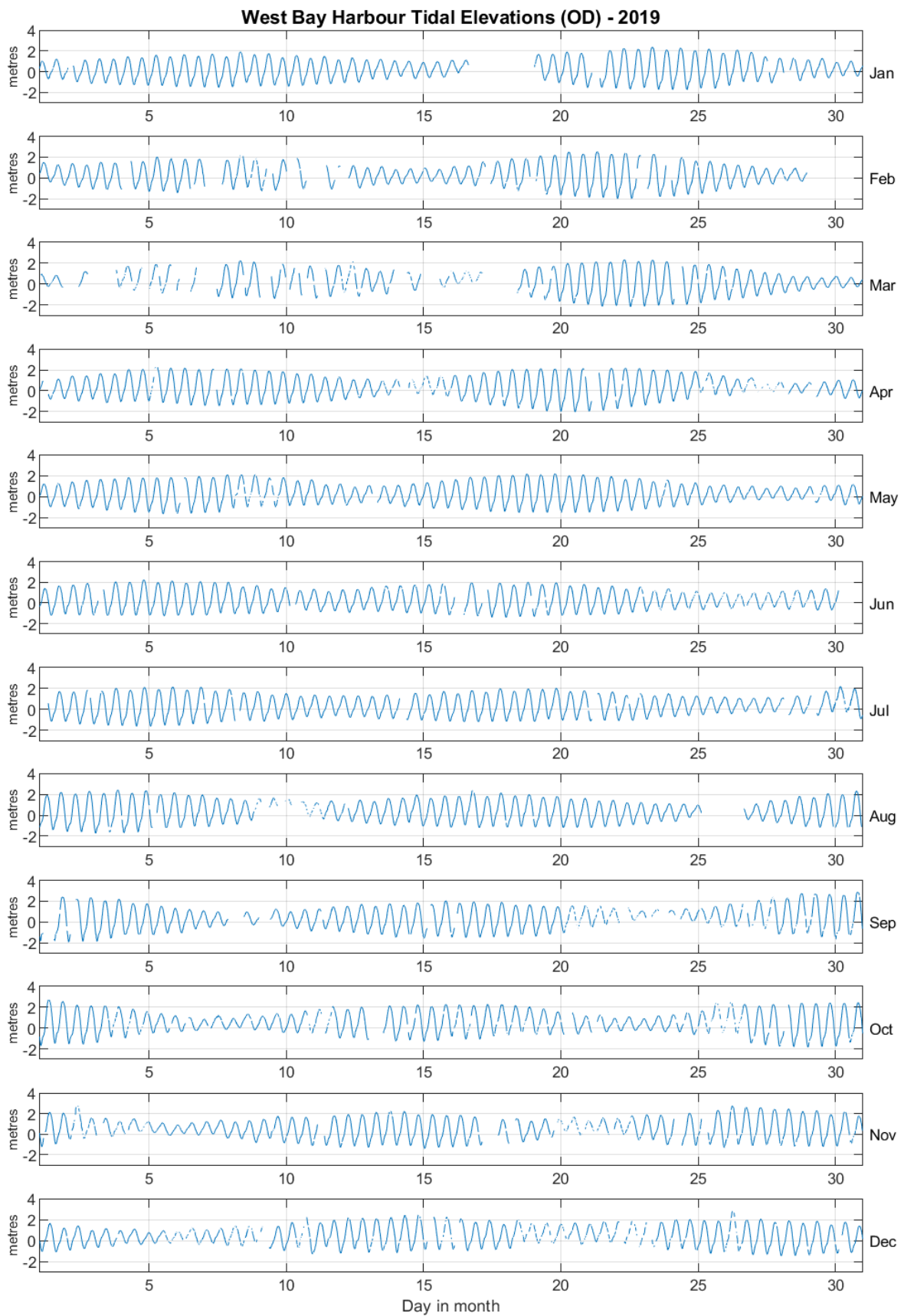
Figure 2: West Bay Harbour tidal elevations for 2019 relative to Ordnance Datum
