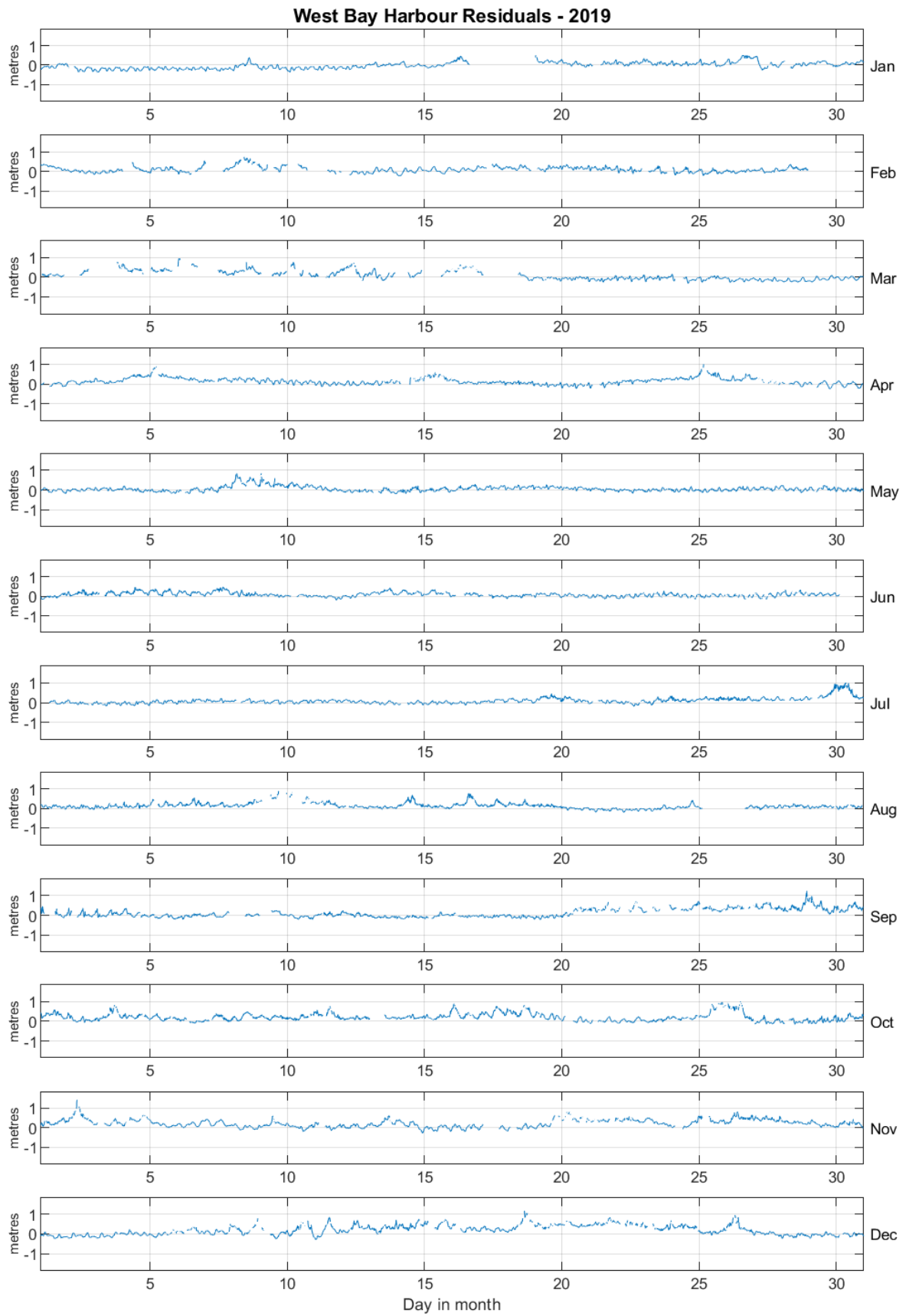
Figure 1: West Bay Harbour residuals for 2019
