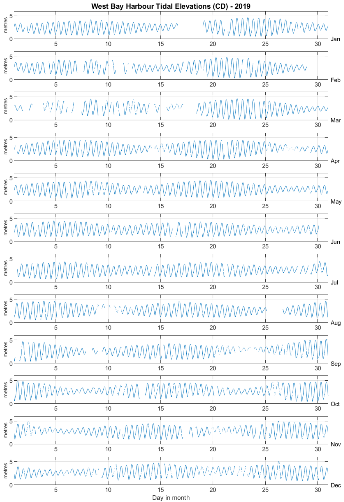
Figure 3: West Bay Harbour tidal elevations for 2019 relative to Chart Datum
